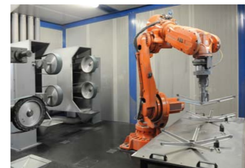
Department of Sharpening Polishing with the use of robotics
