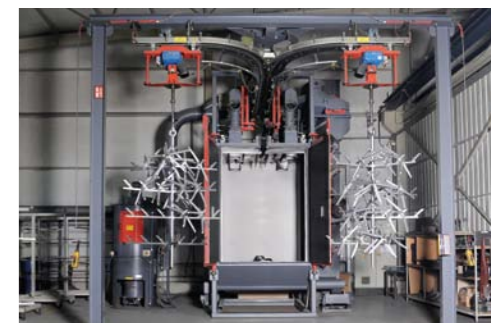
Surface processing with shot blasting
